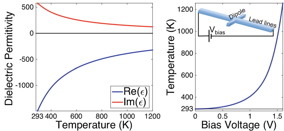
Fig. 1 a Variation of the real and imaginary part of the dielectric constant of nickel with temperature at \lambda = 10.6\mu\text{m} . b Temperature of the dipole antenna as a function of the bias voltage, V_b . The inset shows a sketch of how V_b can be applied to the dipole antenna
