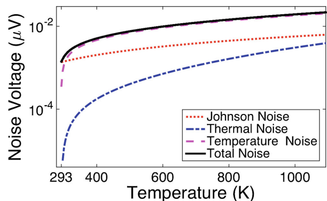
Fig. 5 Semilog representation of the contribution to the noise vs. temperature of three noise mechanism applicable to the distributed bolometer optical antenna. The solid line represents the total noise of the device
