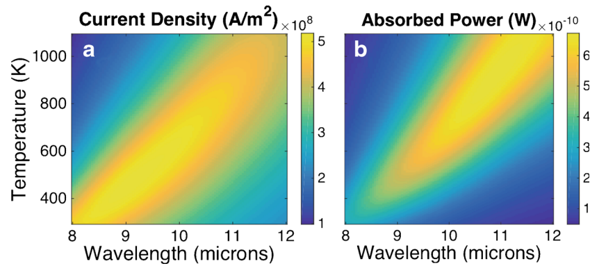
Fig. 3 Current density flowing through the center of the dipole antenna ( a ) and total dissipated power at the antenna volume ( b ) as a function of wavelength and temperature. The current is calculated to model an antenna-coupled MIM diode, and the total dissipated power
