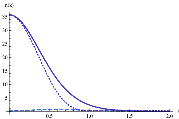
Figure 1: Occupation numbers for temporal (continuous line) and longitudinal (dashed line) photons in the out region vs. k in \eta_0^{-1} units. We also show the analytical approximate solution (dotted line) given in the main text.
