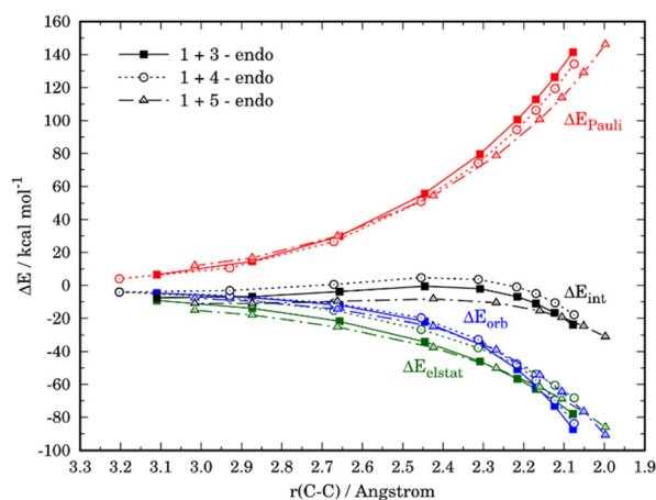
Fig. 7 Comparative energy decomposition analyses of the Diels–Alder for the endo -pathways of the cycloaddition reactions between maleic anhydride ( 1 ) and furan ( 3 ) (solid lines), 3-nitrofurane ( 4 ) (dotted lines), and N,N -dimethylfuran-3-amine ( 5 ) (dashed lines).
