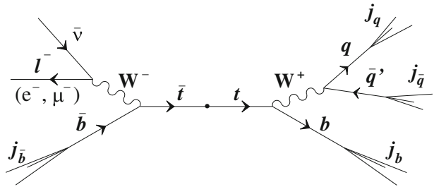
Fig. 2 Schematic example of the top and anti-top decays in the lepton plus jets channel
