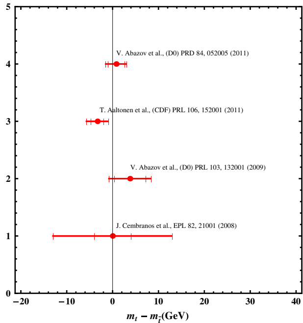
Fig. 4 Evolution of the constraints on the mass difference between top and anti-top quarks. The present improvement with respect to the first analysis in 2008 [53] is one order of magnitude, due fundamentally to a better control on systematic uncertainties
